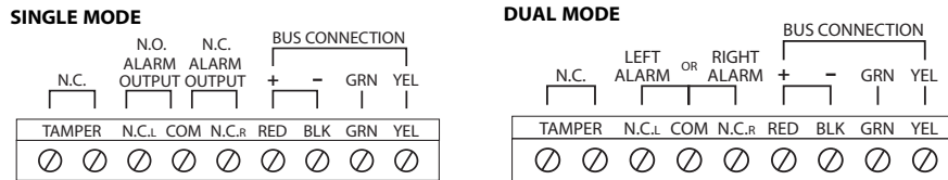
Figure 1: Wiring Methods
