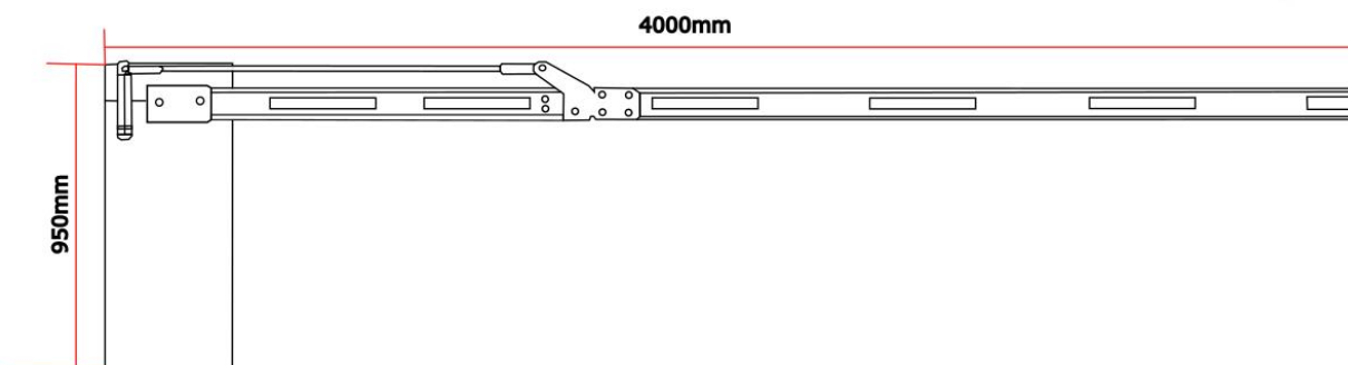
180° folding arm
