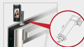
Mounting Bracket
